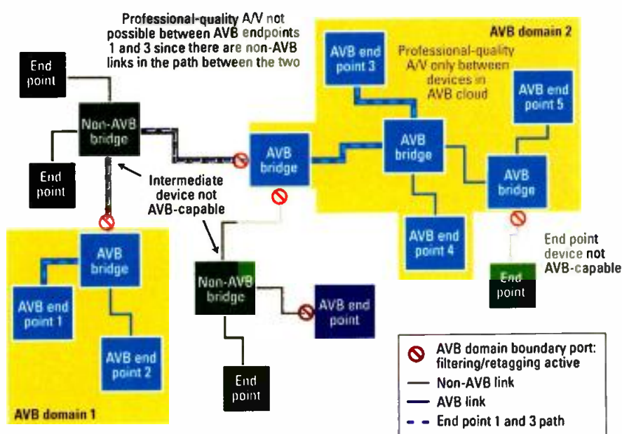
Figure 1. AVB will require AVB-aware bridges and end points in order to operate correctly. This means that if you want to use it, you will need to carefully qualify devices on your network to ensure they meet AVB standards.
