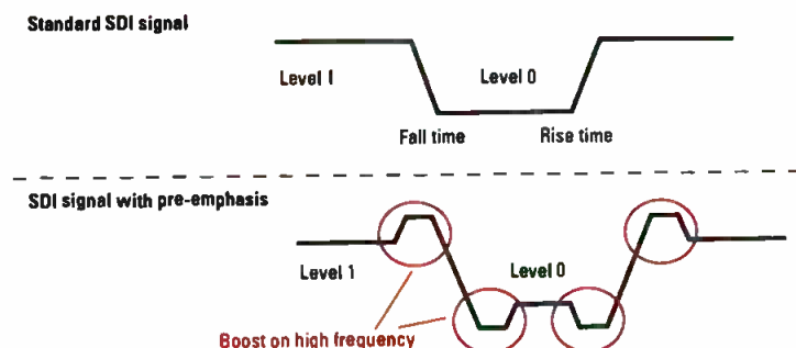
Figure 4. Digital signals without pre-emphasis (top) and with pre-emphasis (bottom)
