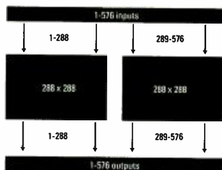
Figure 5. Blocking 576 x 576 router
